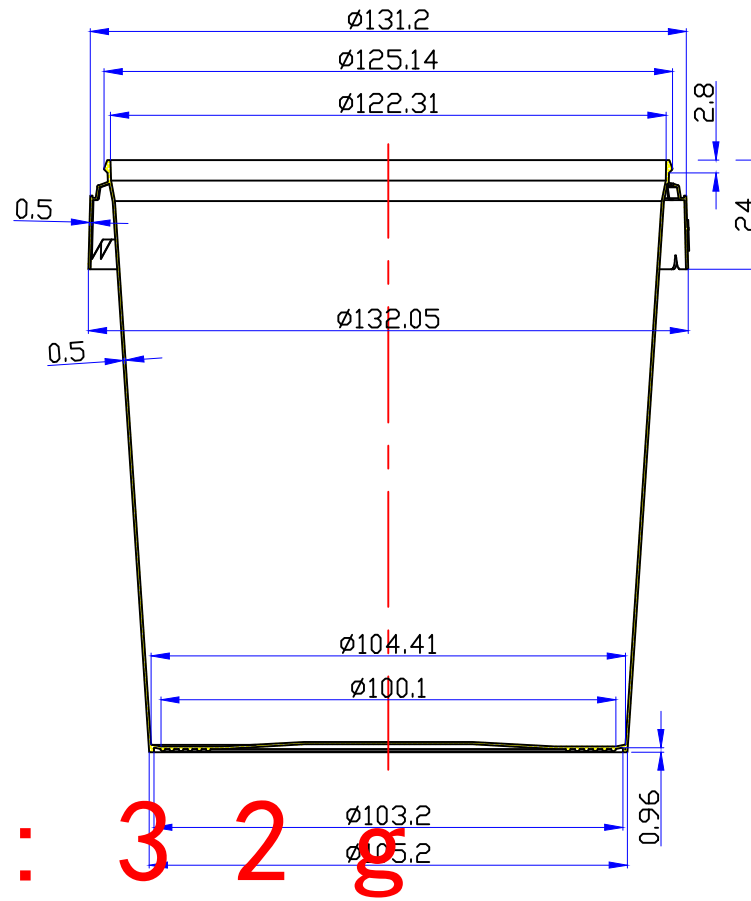
SECTION C-C
